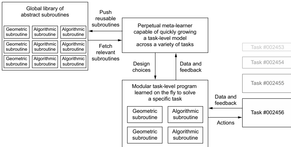
Figure 14.13 A meta-learner capable of quickly developing task-specific models using reusable primitives (both algorithmic and geometric), thus achieving extreme generalization
