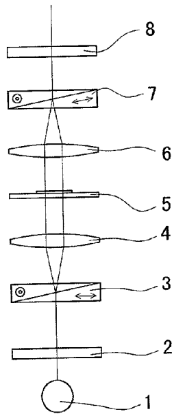
FIG.1 PRIOR ART
