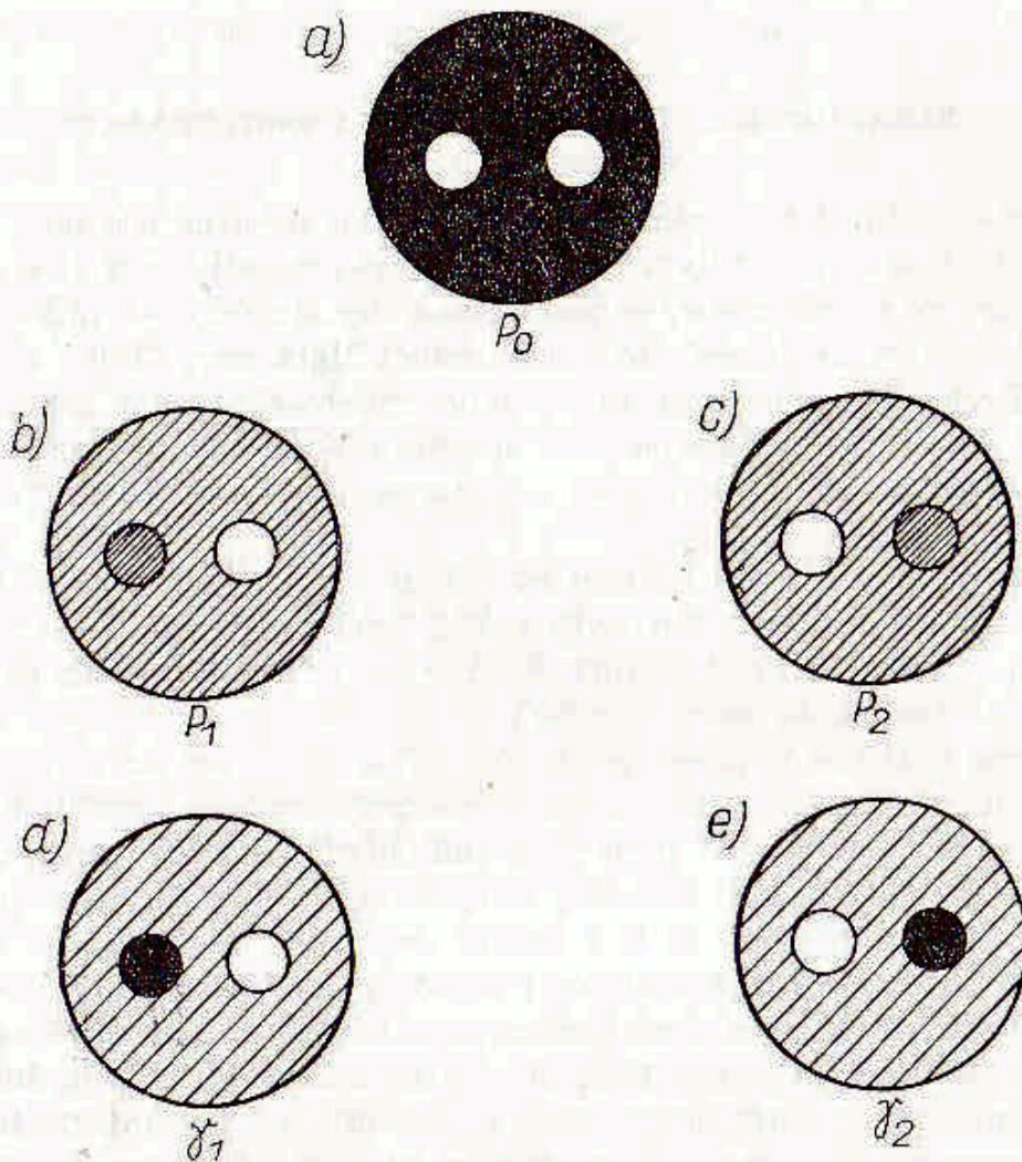
Fig. 40: Simultaneous measurement of optical path difference and light transmittance a) Zero position of birefringent prism; b) Compensation of phase shift in L.H. image; c) Compensation of phase shift in R.H. image; d) L.H. image amplitude compensation; e) R.H. image amplitude compensation
