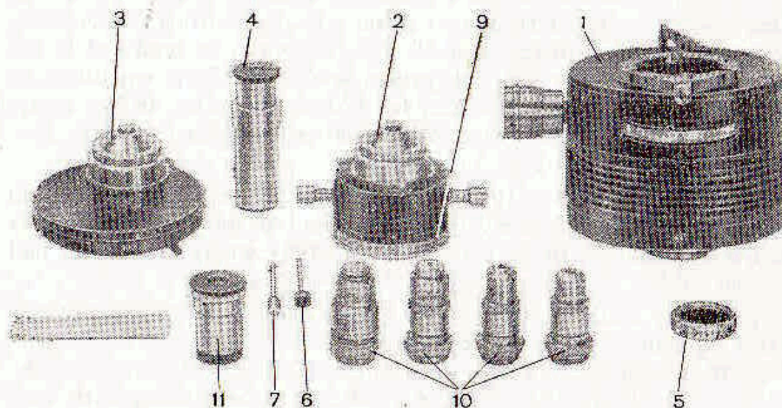
Fig. 10: Basic components of a polarizing interference system
