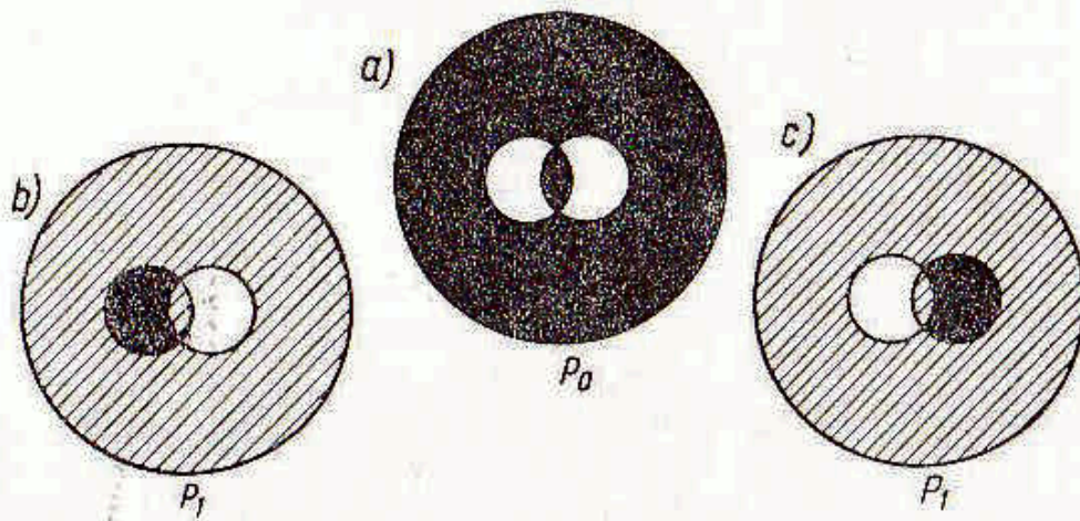
Fig. 27: Optical path difference measured by a method of darkening one of the split images of the object under observation in an uniform interference field
