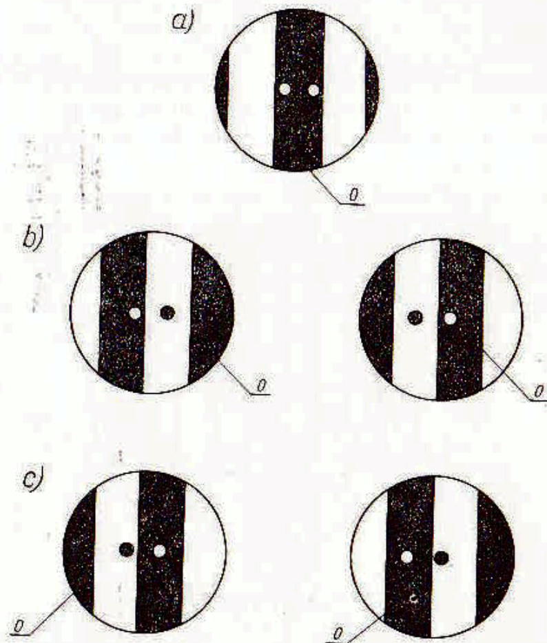
Fig. 26. Optical path difference measured in a fringed interference field with darkening of images and gauging of birefringent prism transversal shift a) Dark zero fringe provided to the centre of image of the object under examination; b) Image of the object being investigated, darkened by a zero interference fringe ( \theta ); c) Another image darkened with the same zero interference fringe ( \theta )
