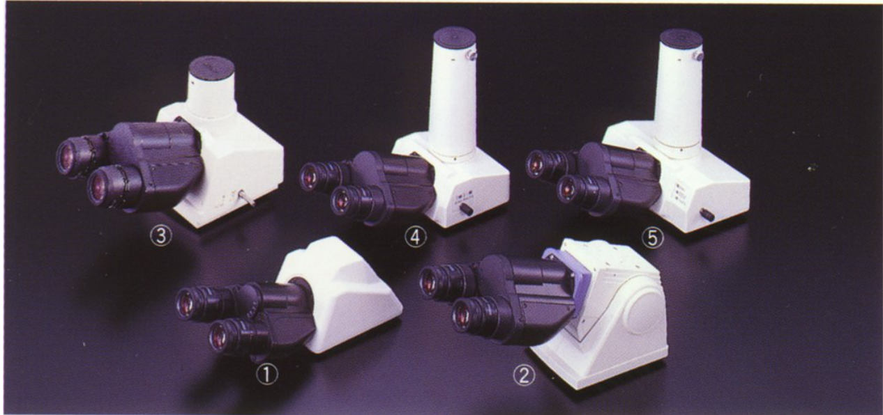
1. Y-TB Binocular Tube, 2. Y-TE Ergonomic Binocular Tube, 3. L-TI2 Erect-image Trinocular Tube, 4. Y-TF Trinocular Tube, 5. Y-TT Trinocular Tube TUW
