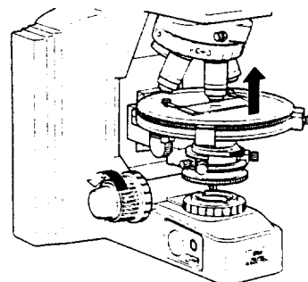
Direction of coarse/fine focus knobs and stage vertical motion
